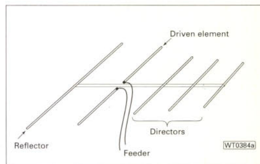
Fig. 2a & b: Yagi antenna (above)- Polar diagram of a Yagi antenna system (below).
