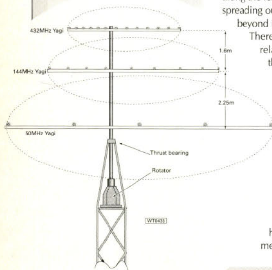
Fig. 2: Putting the lowest band antenna nearest the thrust bearing reduces the strain on the system due to wind loading.
